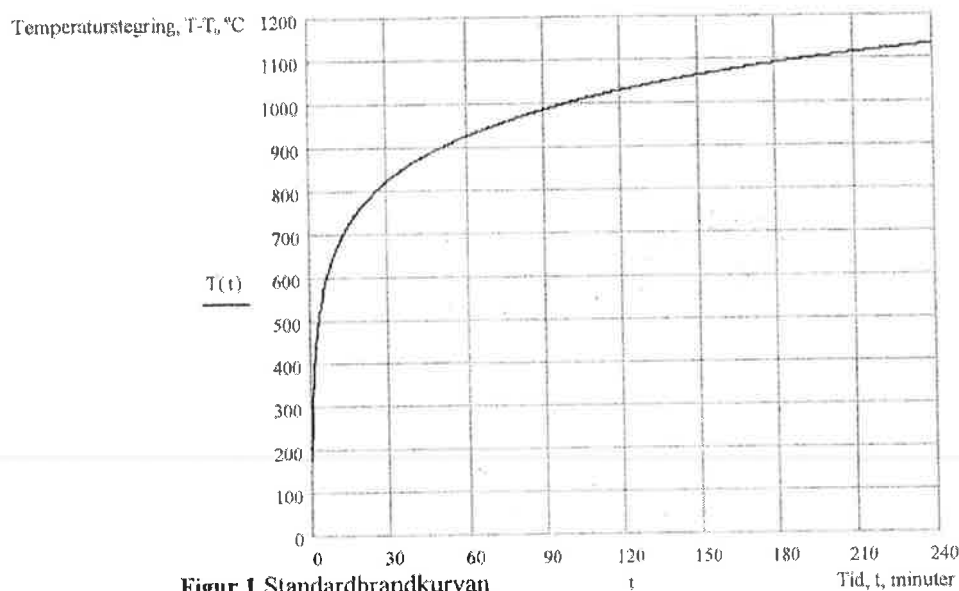
Figur 1 Standardbrandkurvan
